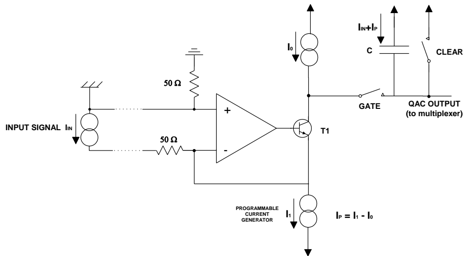
Fig. 2.3: QAC section
