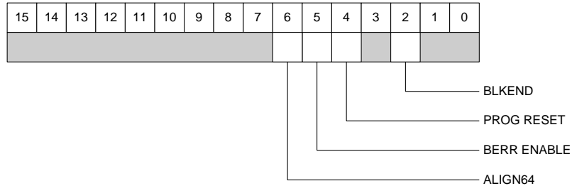
Fig. 4.18: Control Register 1
