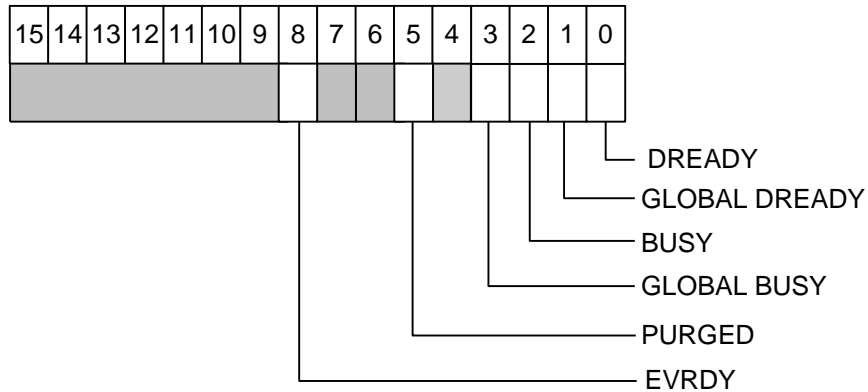
Fig. 4.17: Status Register 1
