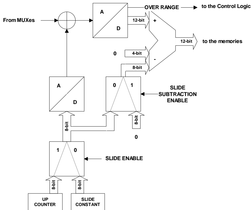
Fig. 2.4: Block diagram of the sliding scale section
