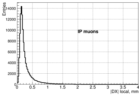
Figure 12. |DX| local for IP muon hits
