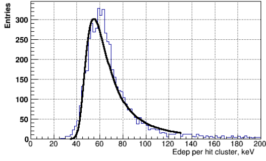
Figure 6. Energy deposition for IP muons
